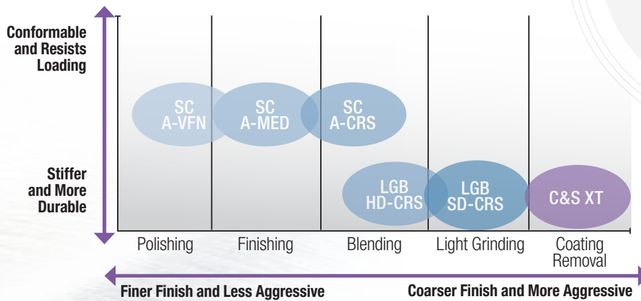
Scotch-Brite™ Disc Performance Comparison
