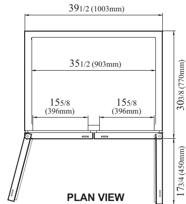
PLAN VIEW
