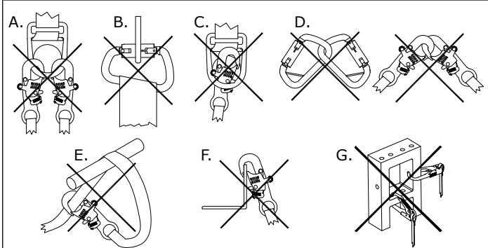
Figure 6 – Inappropriate Connections
