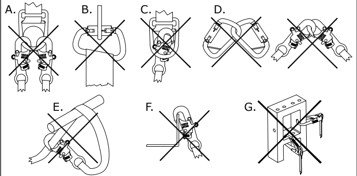
Figure 4 - Inappropriate Connections
