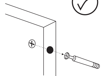
ALIGNED CAM LOCK:
