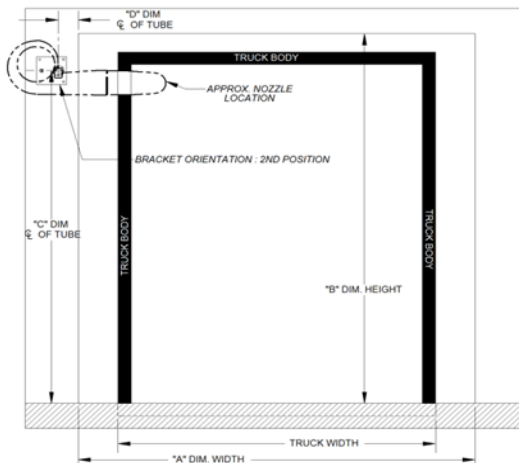
10' x 10' Left Side Mount
