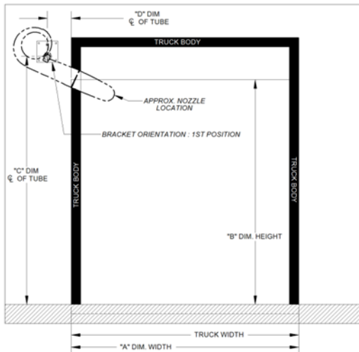
8' x 8' Left Side Mount
