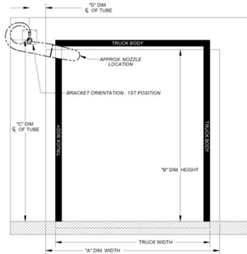
9' x 9' Left Side Mount
