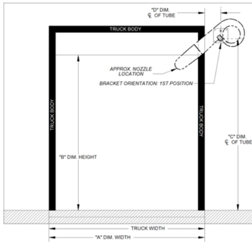
8' x 8' Right Side Mount
