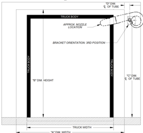
10' x 10' Right Side Mount
