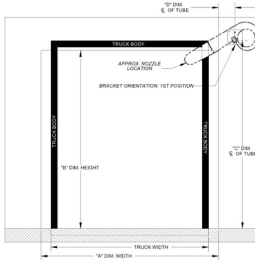
9' x 9' Right Side Mount
