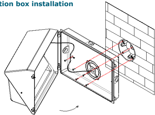
Junction box installation
