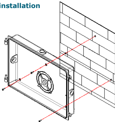
Direct wall-mount installation
