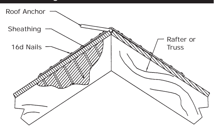
Figure 7 - Anchor Installation
