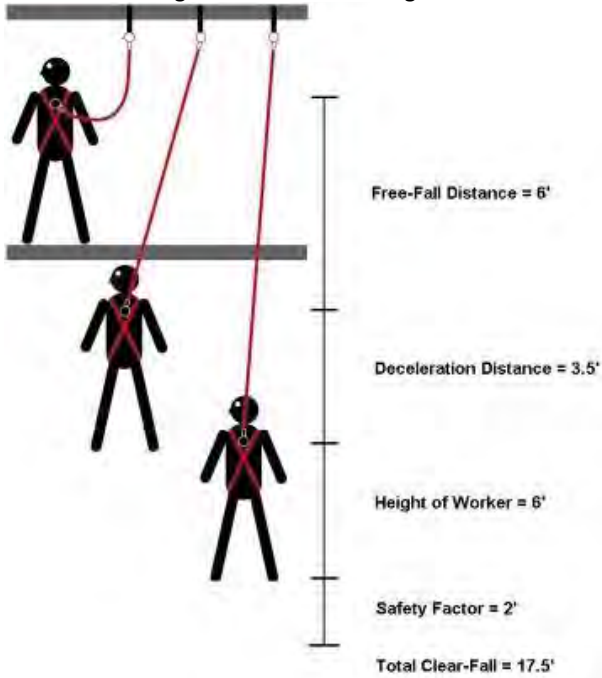
Figure 2.1: Clear-Fall Diagram
