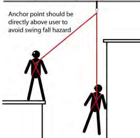
Figure 2.2: Swing-Fall Diagram
