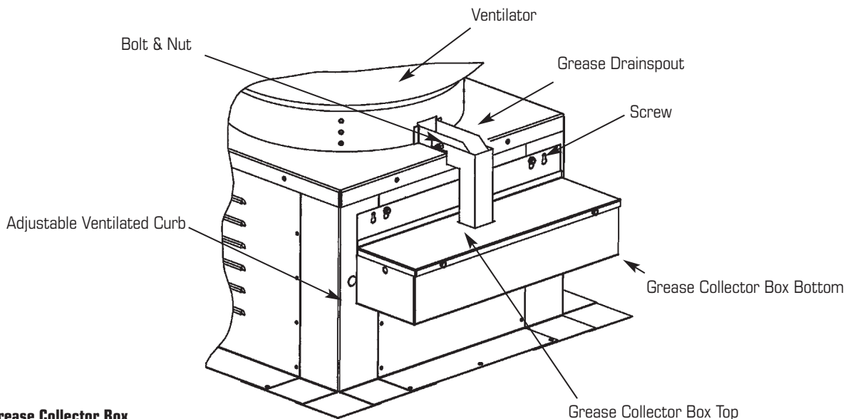
Figure 1 – Grease Collector Box
