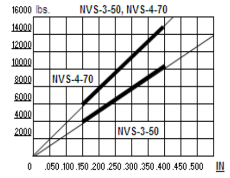
LOAD vs DEFLECTION
